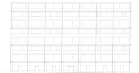
West Elevation
